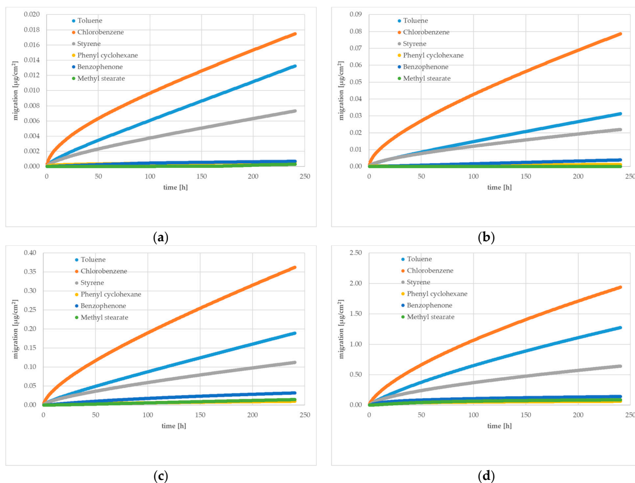
Figure 1. Experimentally determined gas phase migration kinetics of from HIPS at 5 °C (a), 20 °C (b), 40 °C (c) and 60 °C (d). Spiking levels for the different substances are indicated in Section 2.4.
